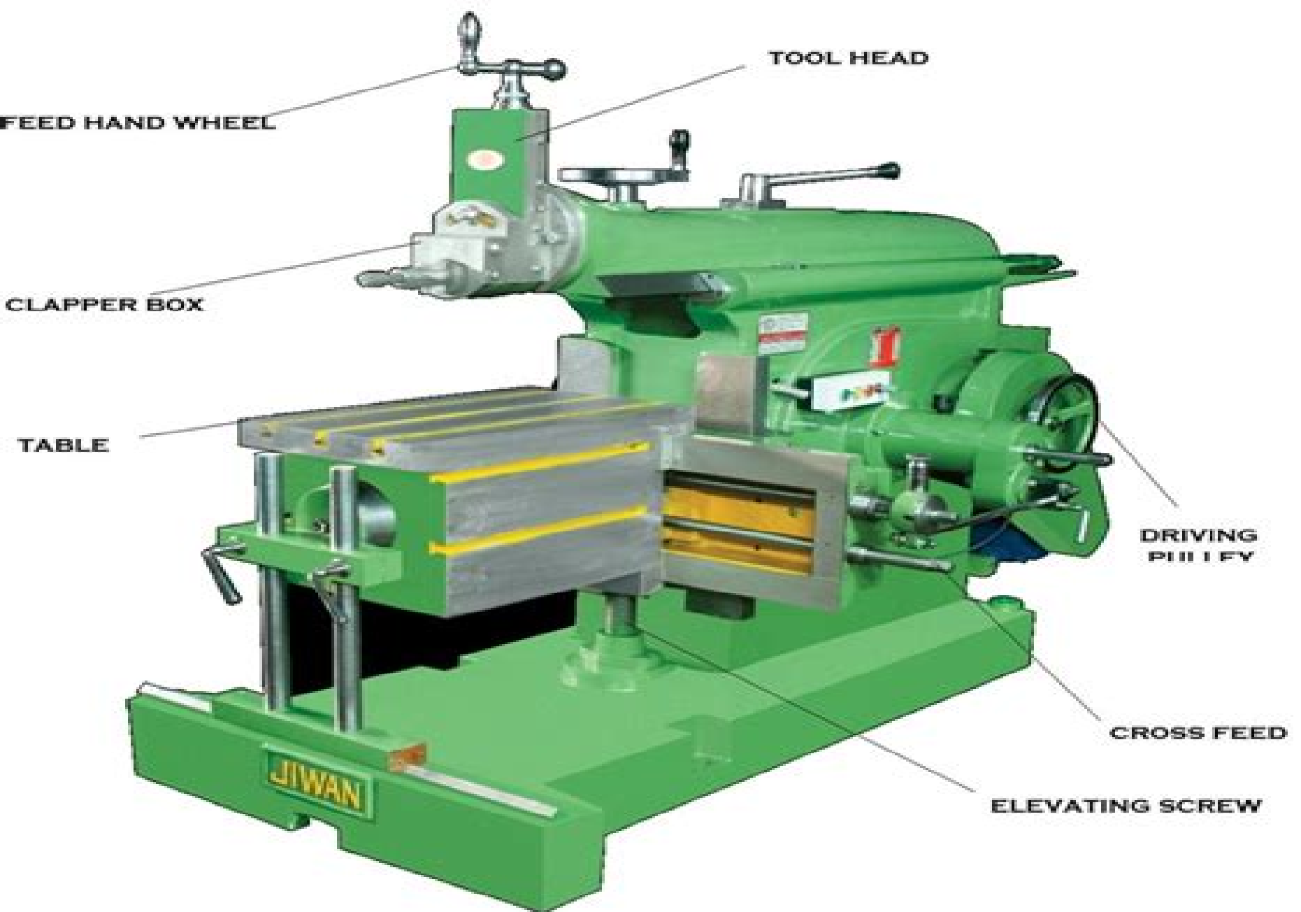
PARTS OF SHAPER MACHINE
