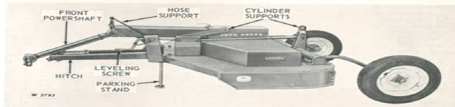
John Deere 507 Pull-Type Gyramor Rotary Cutter (Manufactured 1959- )
