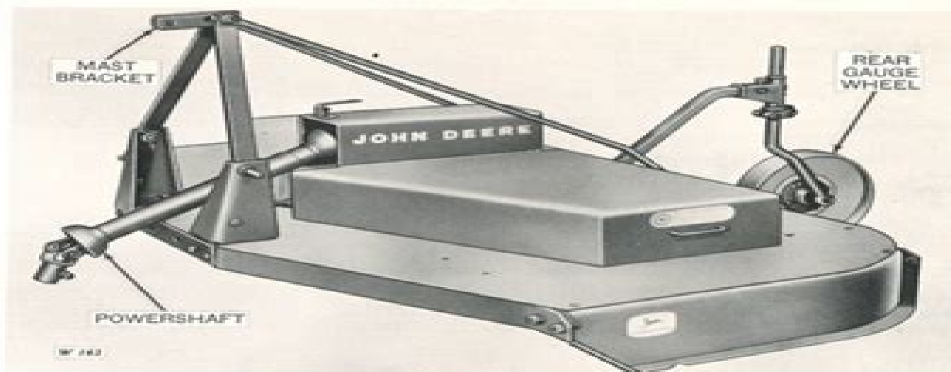
John Deere 507 Integral Gyramor Rotary Cutter Equipped with Rear Gauge Wheel (Manufactured 1959- )
