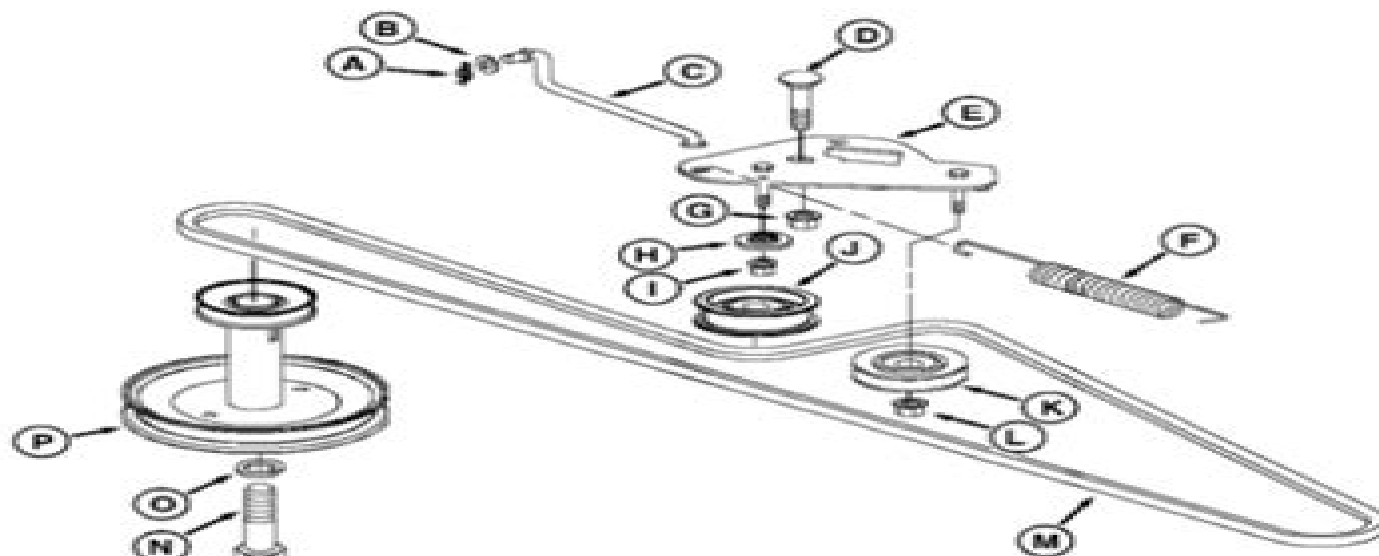
GXT002881-UN: Drive Components - X105
