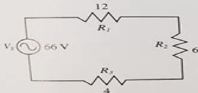
Figure 19-7. Circuit for problem 2.
