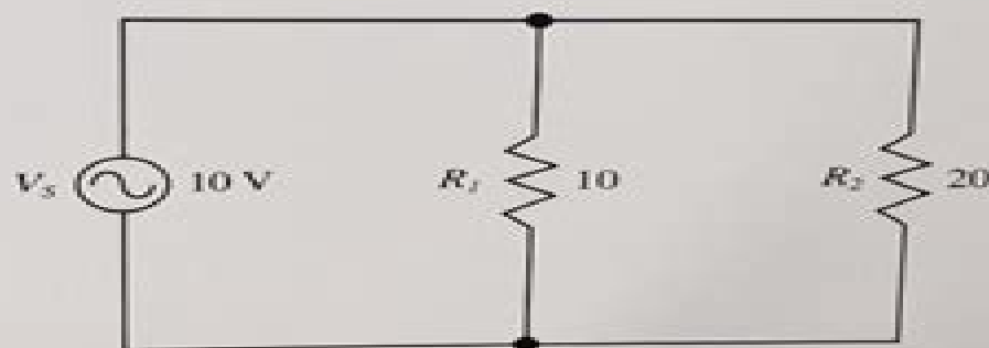
Figure 19-8. Circuit for problems 6 and 8.
