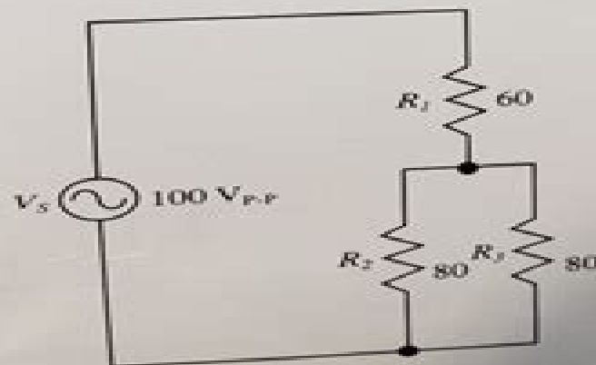
Figure 19-9. Circuit for problem 10.
