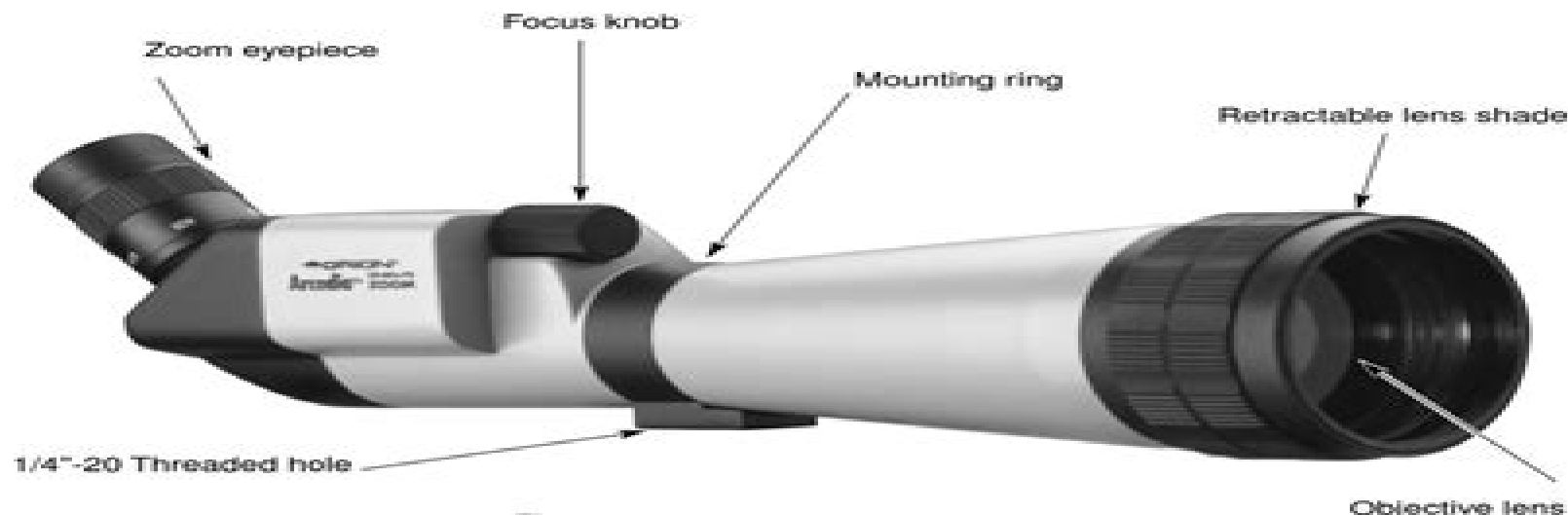
Figure 1. The Arcadia Zoom Spotting Scope
