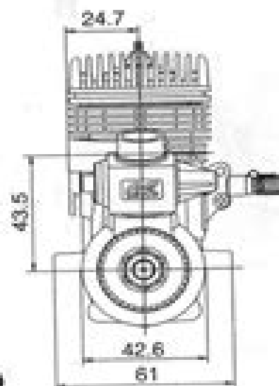
Dimensions(mm)
