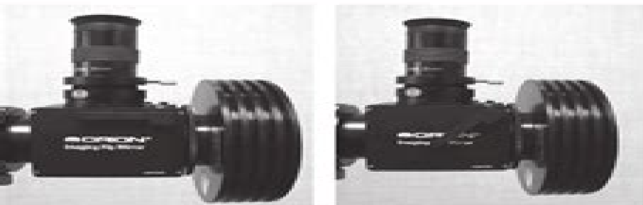
Figure 5.1. Lever up directs the light path to the CCD camera.
