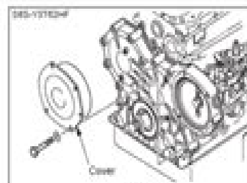
Installing cover
