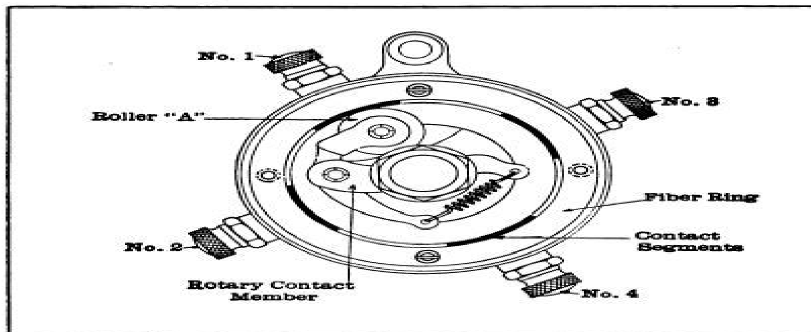
Fig. 19.—Parts of the Ford Ignition Timer.
