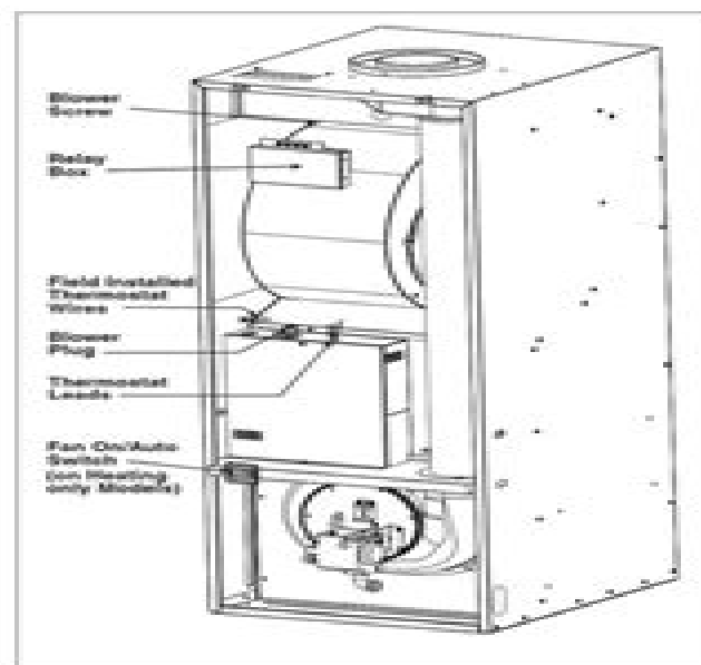
Fig 2. M1* Furnace
