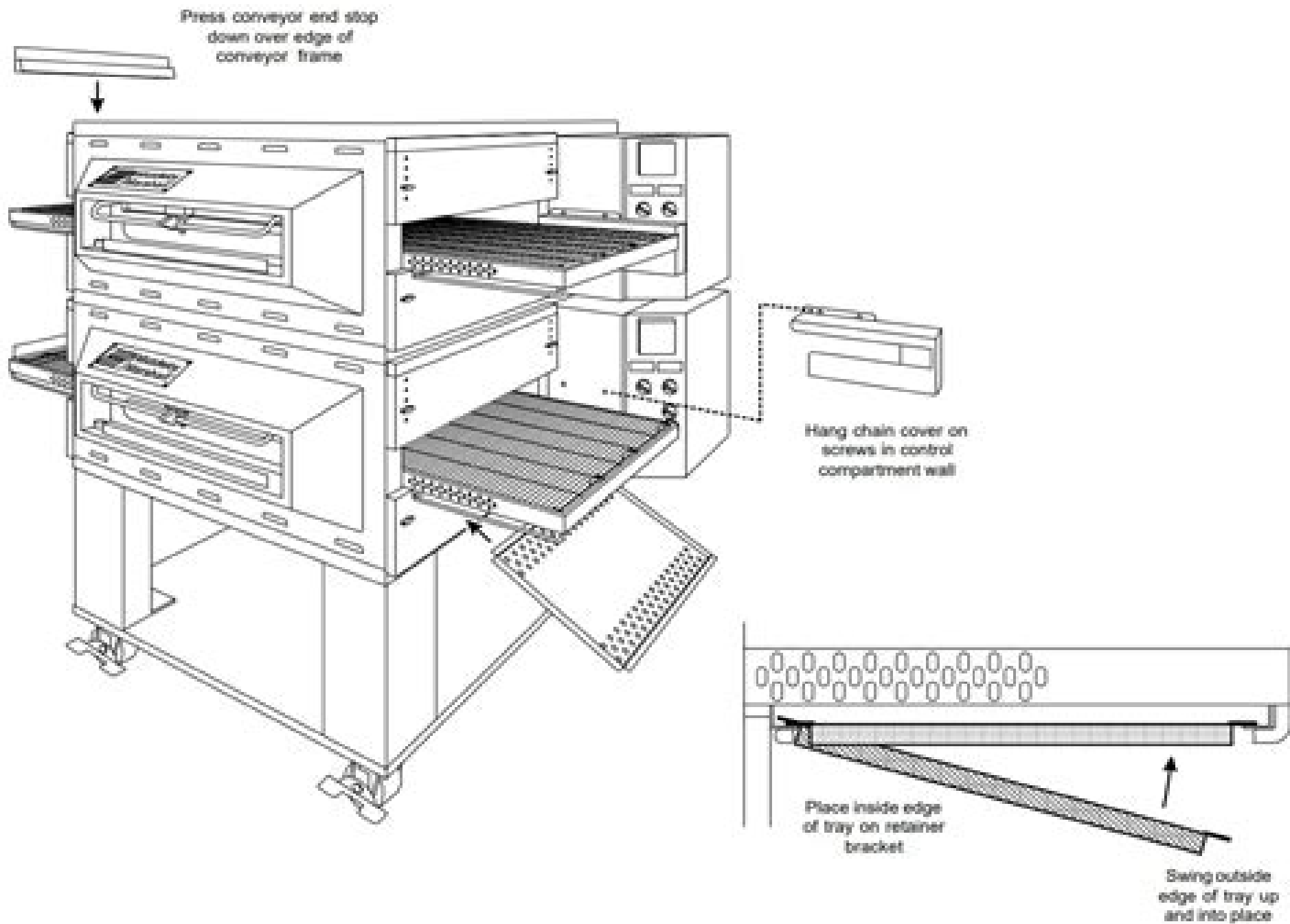
Figure 2-13 - Final assembly
