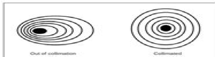
Figure 1: A star test will determine if a telescope's optics are properly collimated. An unfocused view of a bright star through the eyepiece should appear as illustrated on right if optics are perfectly collimated. If circle is unsymmetrical, as in illustration on left, scope needs collimation.
