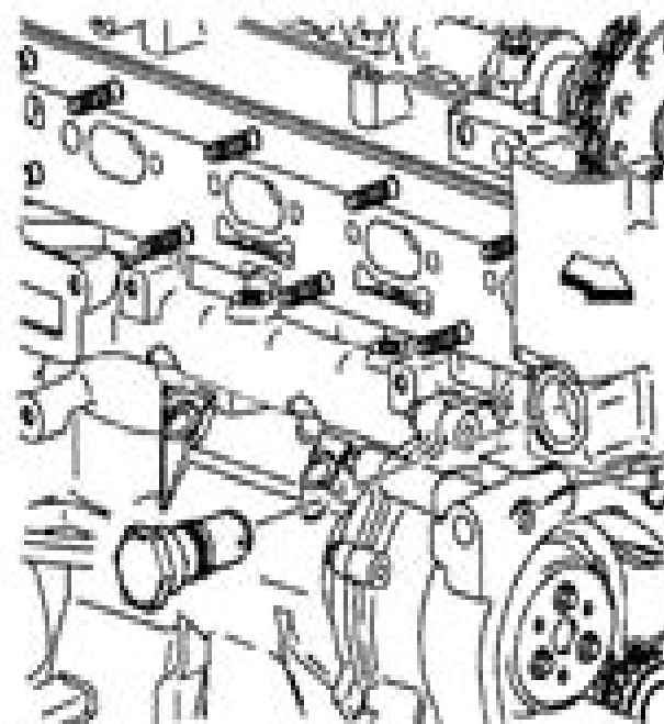
Fig. 124: Installing Timing Chain Tensioner Courtesy of GENERAL MOTORS CORP.
