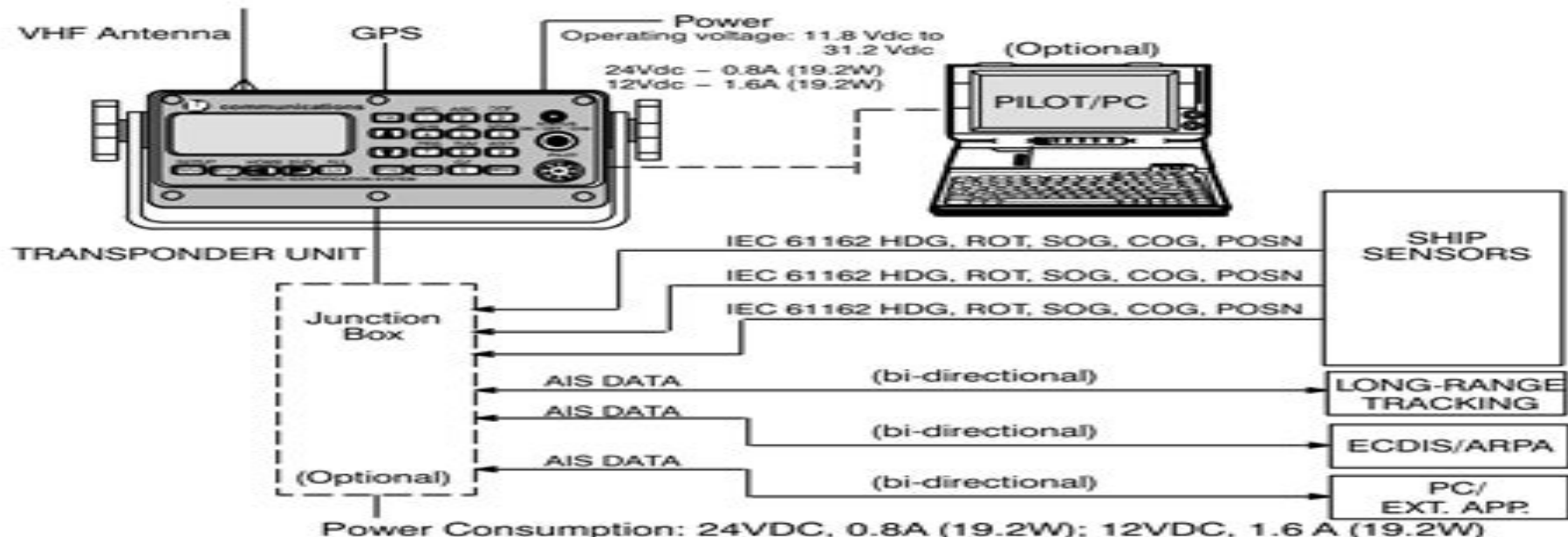
Figure 3-1. AIS Transponder Interconnection Diagram
