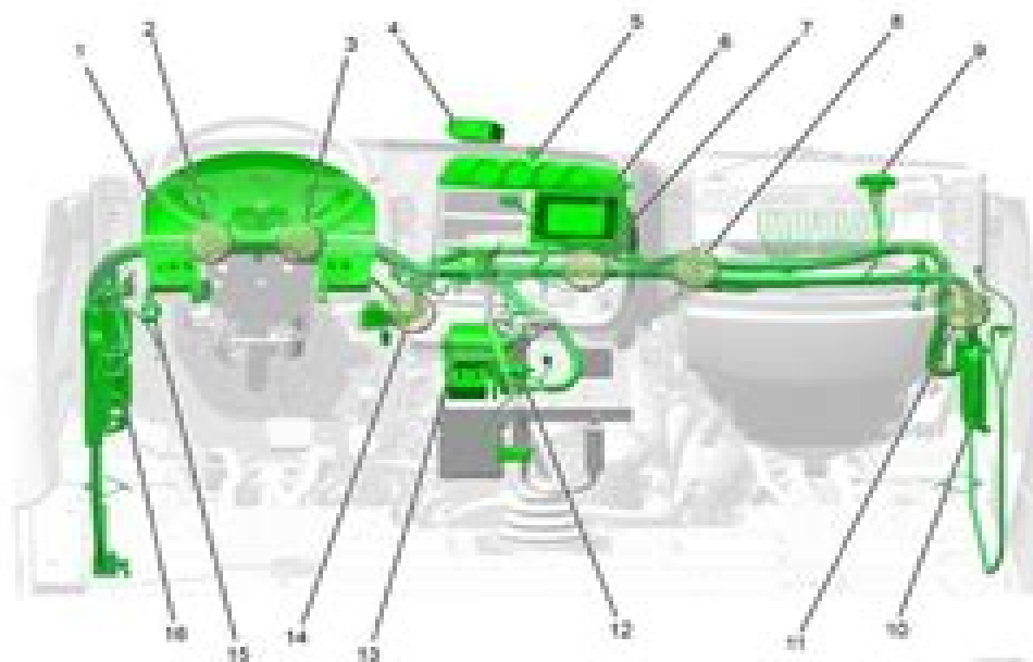
Figure 347 ProStar J1939 dash components
