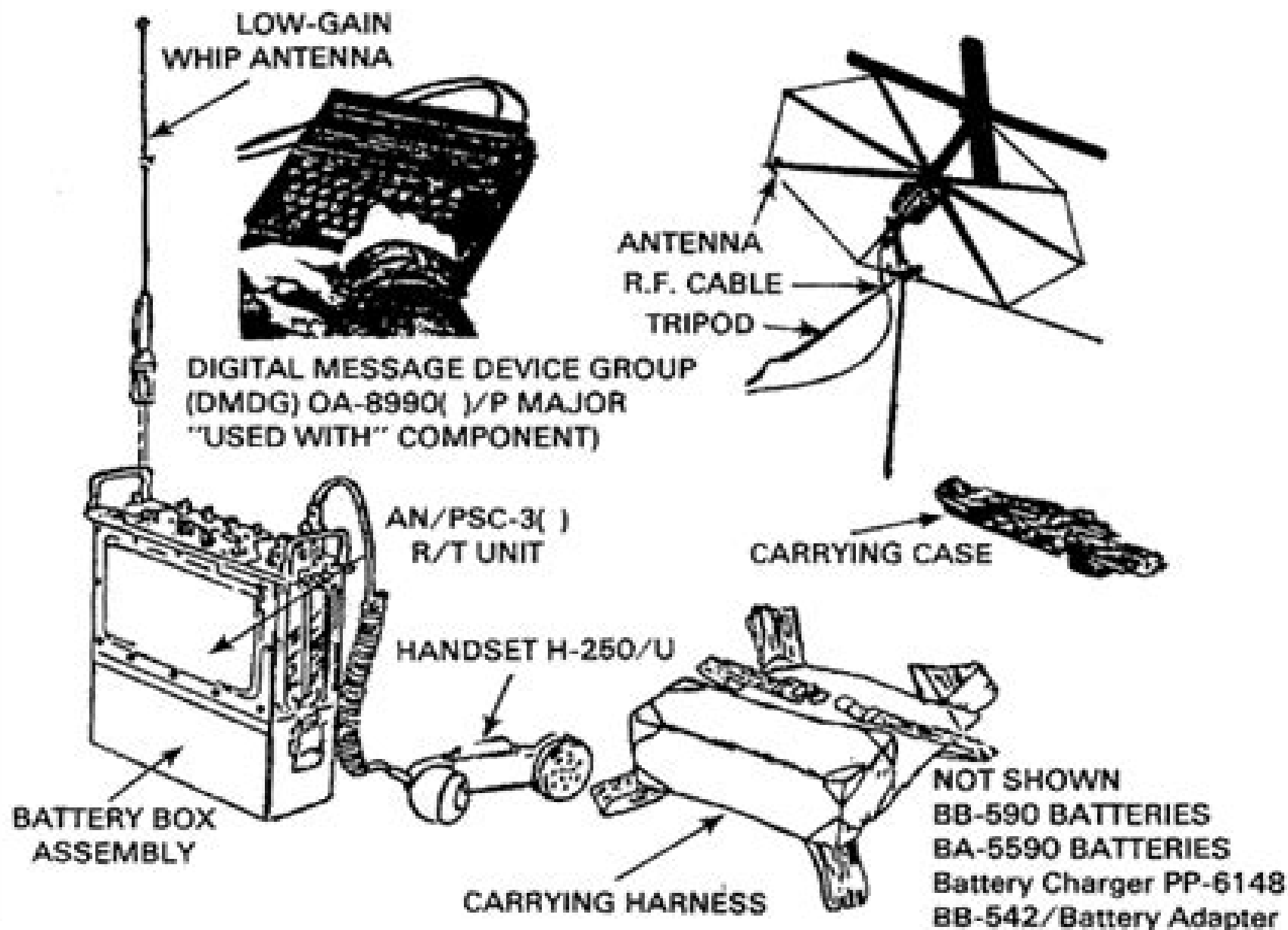
Figure L-4b. Radio Set AN/PSC-3( ) components.
