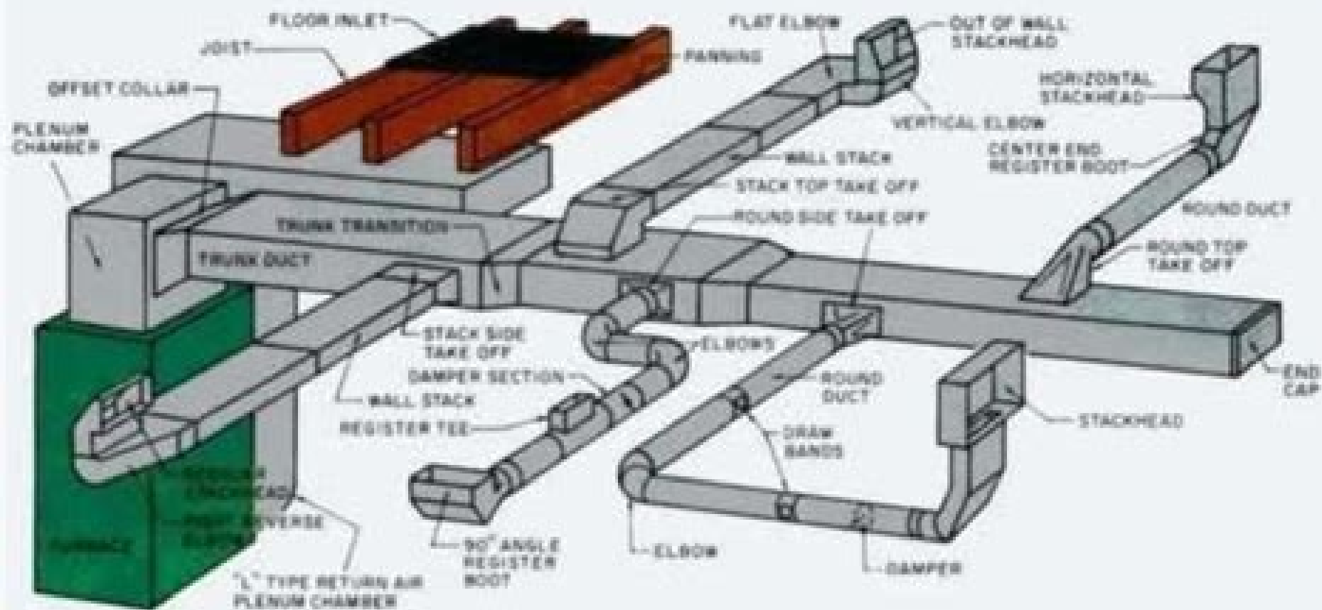
Duct fittings.
