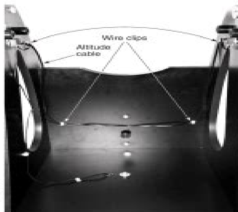
Figure 1: For the SkyQuest XT12 IntelliScope, the routing for the altitude cable should be as shown.
