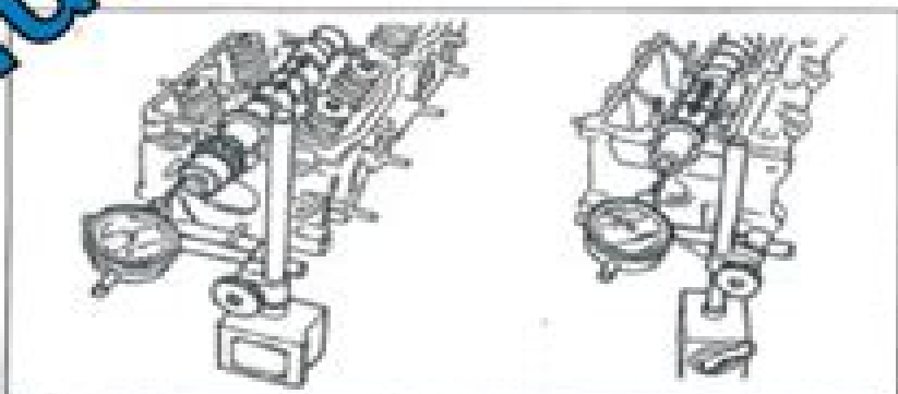
Fig. 1.77 — Checking the camshaft and fuel. On the left for the petrol engine, on the right for the diesel engine.
