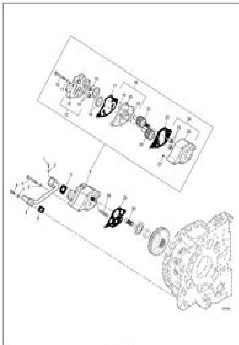
Figure 58. Oil Pump
