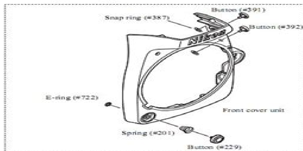
Front cover unit (#824)
