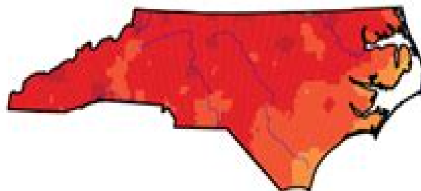
(c) Higher Scenario (RCP8.5), 2041–2060
