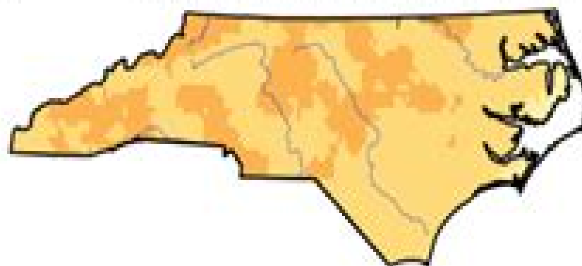
(b) Lower Scenario (RCP4.5), 2041–2060
