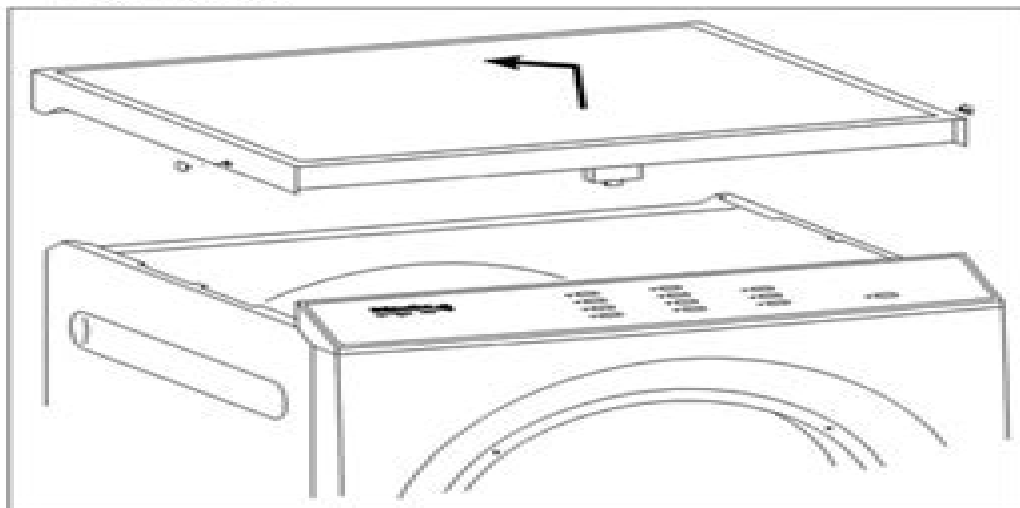
Figure 010-1: Lid Removal
