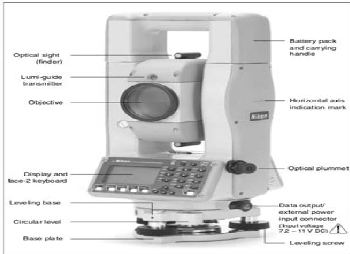
Figure 1.2 Electronic Total Station DTM-502 series - Face-2
