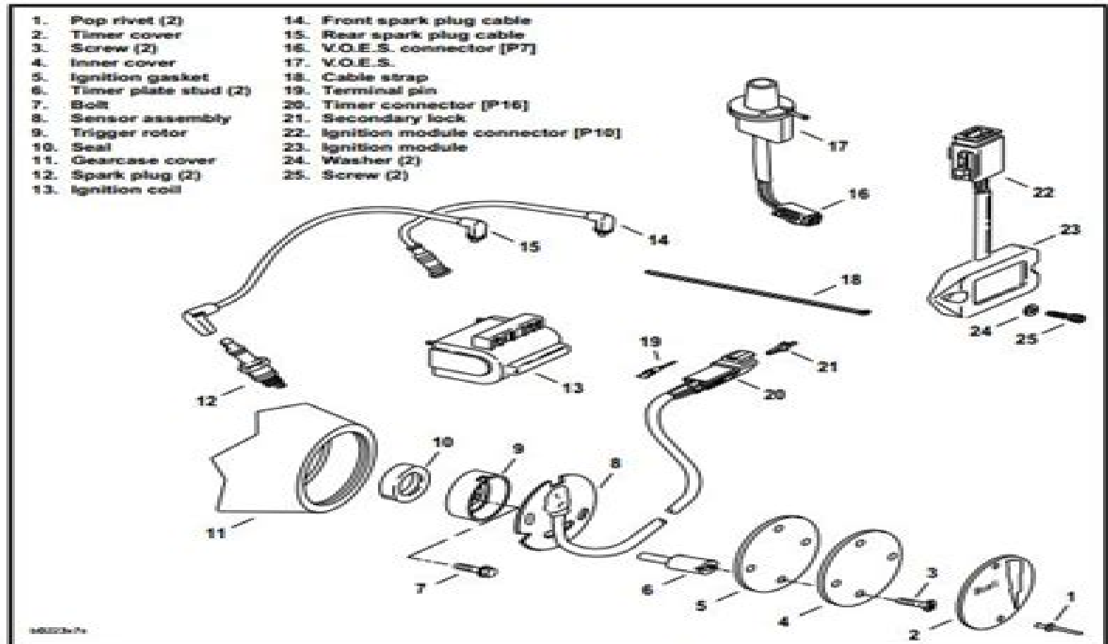
Figure 7-1. Ignition System Components
